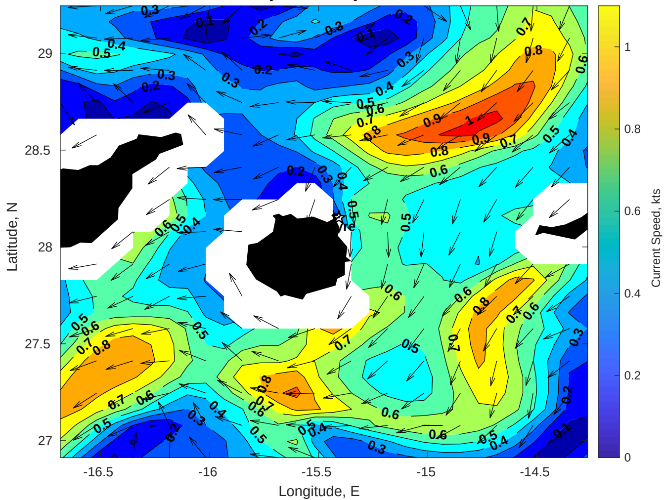
Surface Currents for Gyre at 28-May-2025 00:00:00
