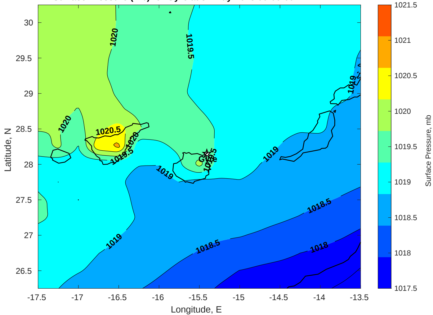
Surface Pressure (mb) for Gyre at 31-May-2025 00:00:00
