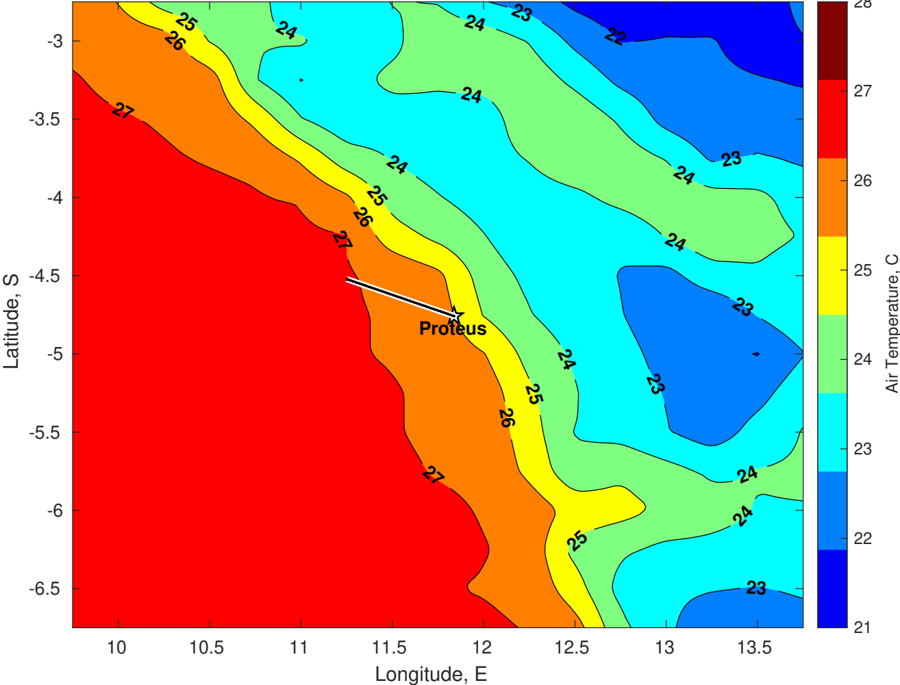
Air Temperature (C) for Proteus at 27-May-2025
