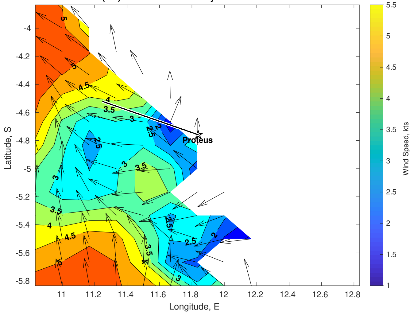
Winds (kts) for Proteus at 27-May-2025 09:00:00
