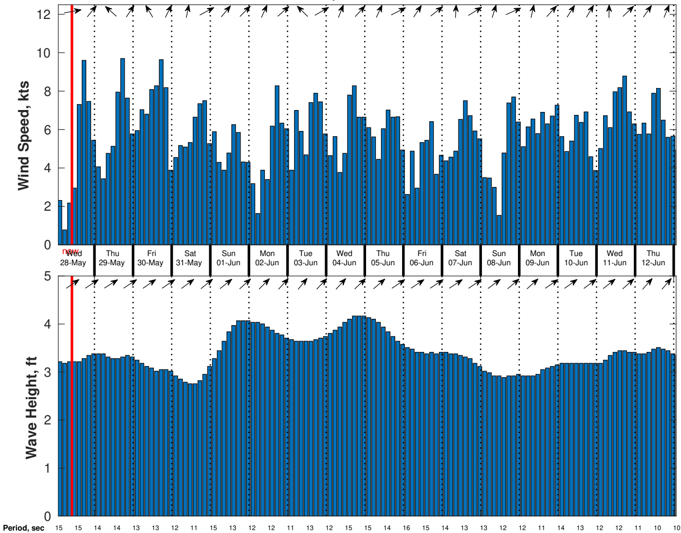
Wind & Wave Forecast for Proteus from 27-May-2025 01:00:00 to 12-Jun-2025 01:00:00
