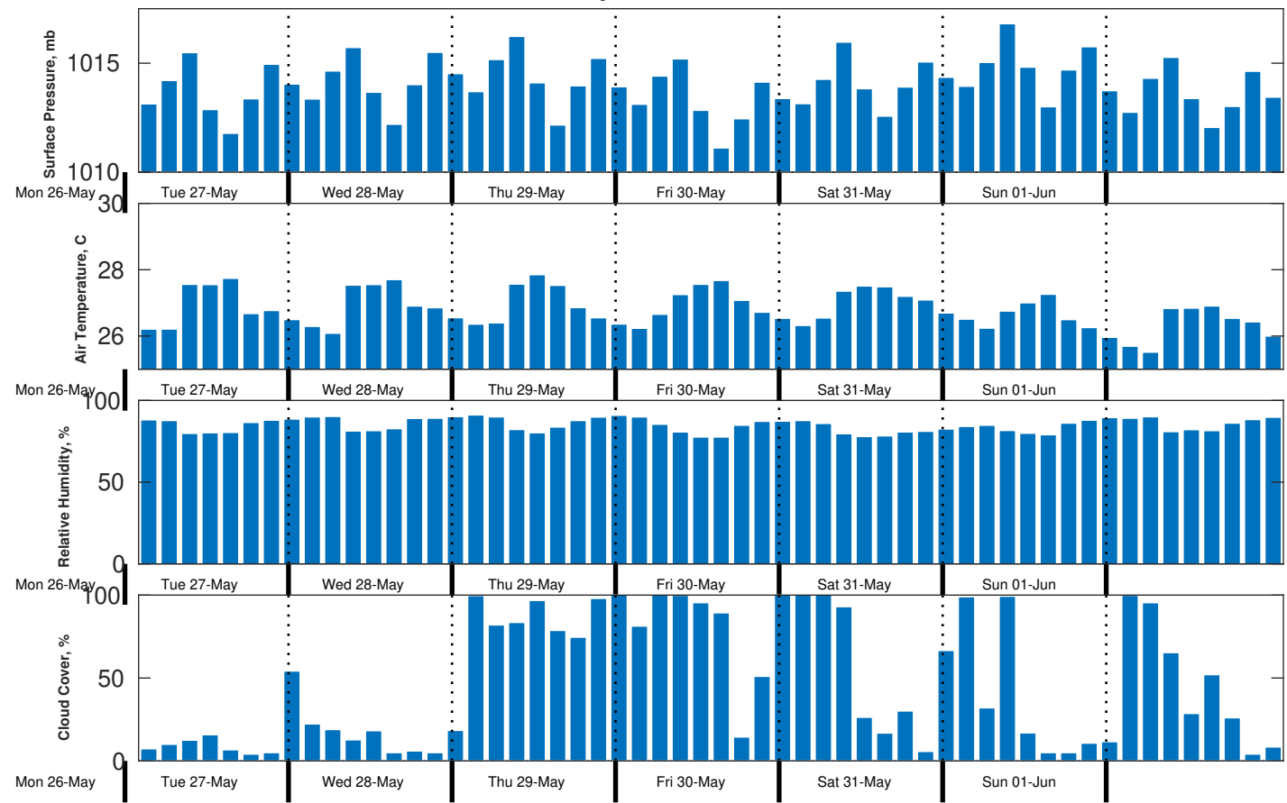
Met Forecast for Proteus from 27-May-2025 00:00:00 to 03-Jun-2025 00:00:00
