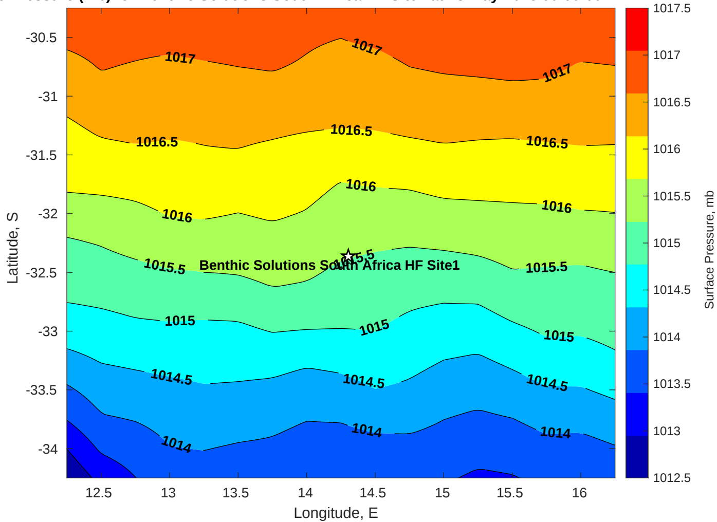
Surface Pressure (mb) for Benthic Solutions South Africa HF Site1 at 28-May-2025 00:00:00
