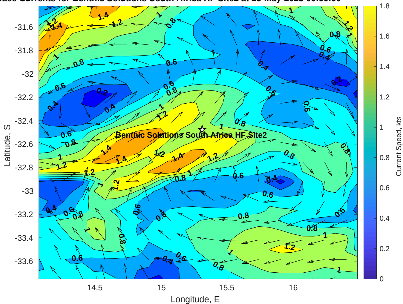
Surface Currents for Benthic Solutions South Africa HF Site2 at 26-May-2025 00:00:00
