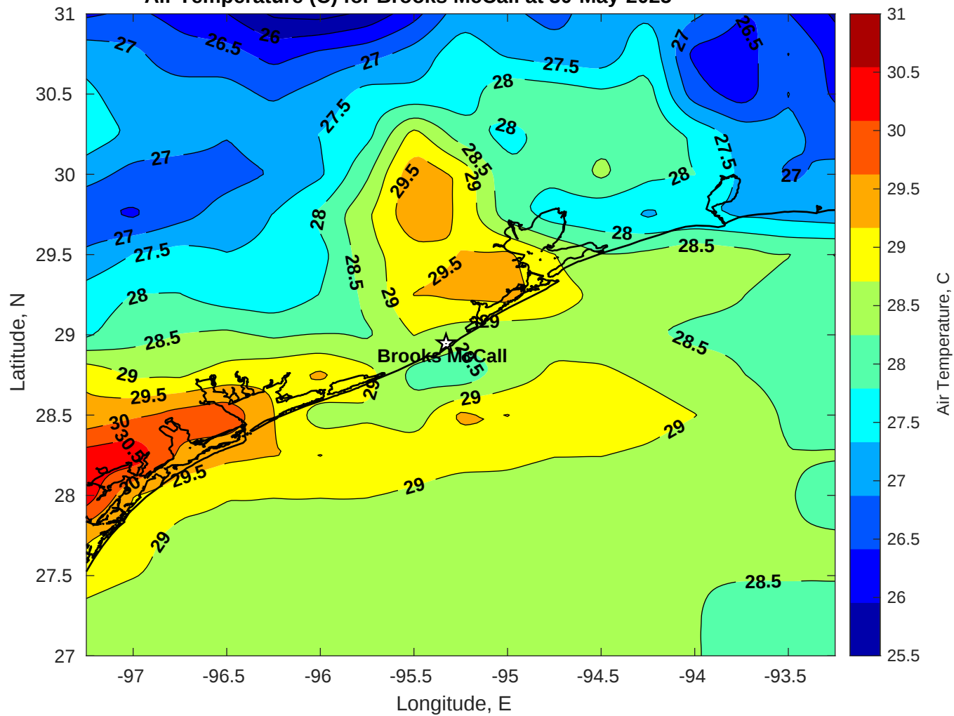
Air Temperature (C) for Brooks McCall at 30-May-2025
