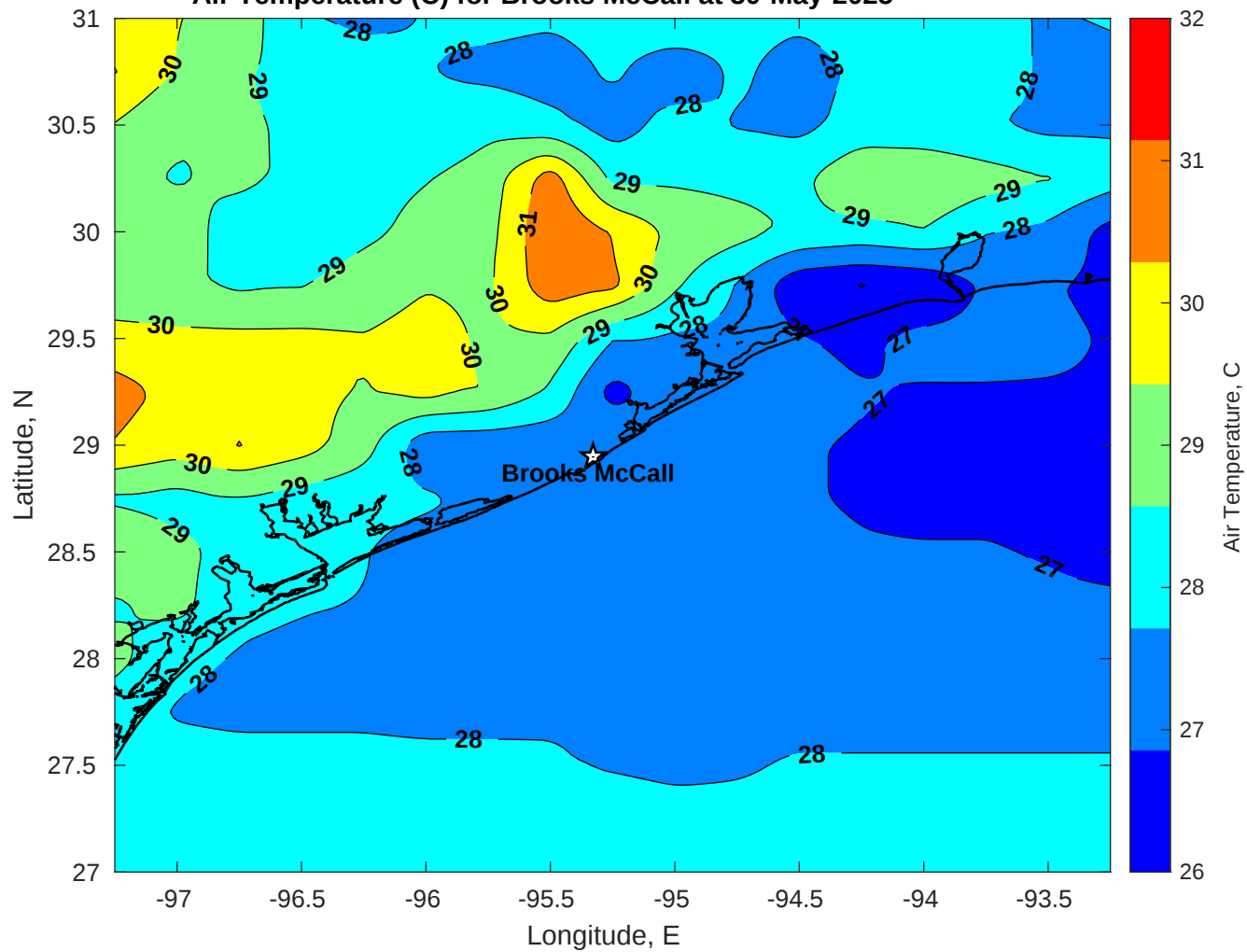
Air Temperature (C) for Brooks McCall at 30-May-2025
