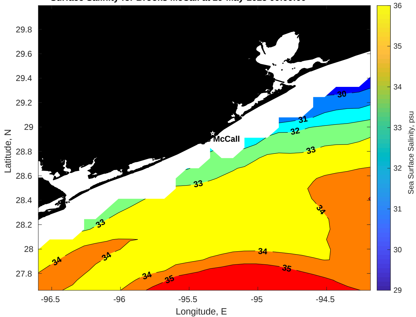
Surface Salinity for Brooks McCall at 29-May-2025 00:00:00
