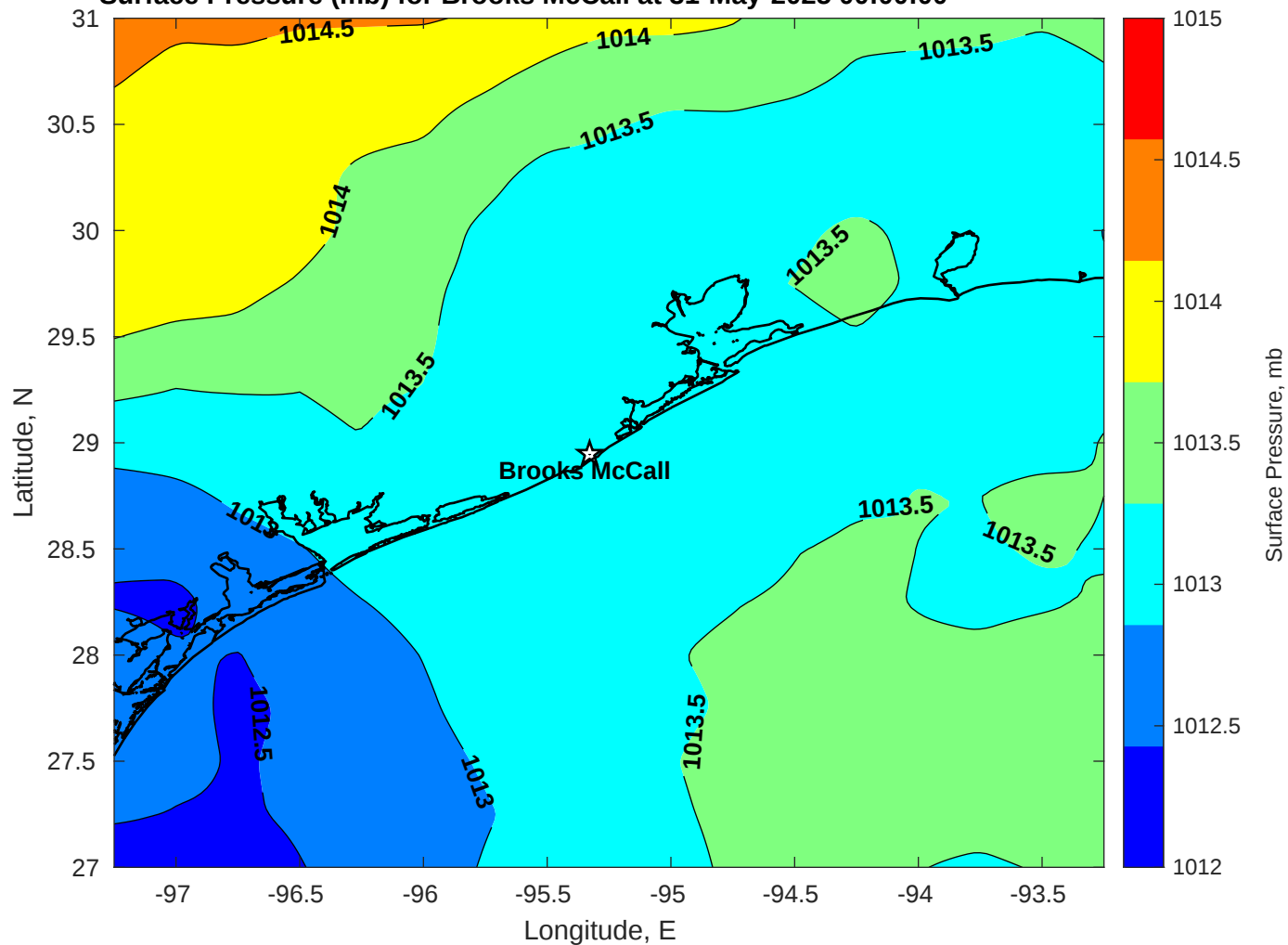
Surface Pressure (mb) for Brooks McCall at 31-May-2025 00:00:00
