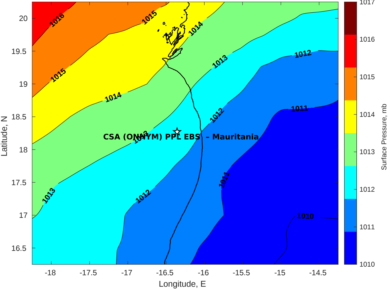
Surface Pressure (mb) for CSA (ONHYM) PPL EBS - Mauritania at 27-May-2025 00:00:00
