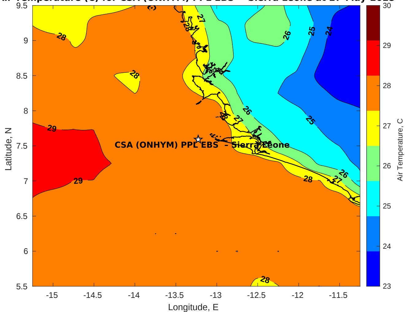
Air Temperature (C) for CSA (ONHYM) PPL EBS - Sierra Leone at 27-May-2025
