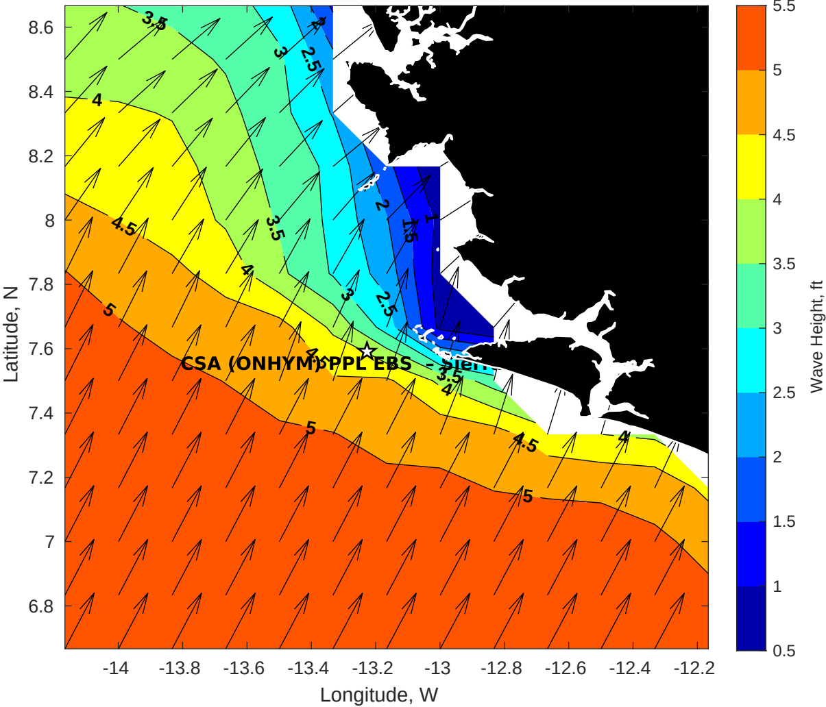
Wave Height (ft) for CSA (ONHYM) PPL EBS - Sierra Leone at 27-May-2025 09:00:00
