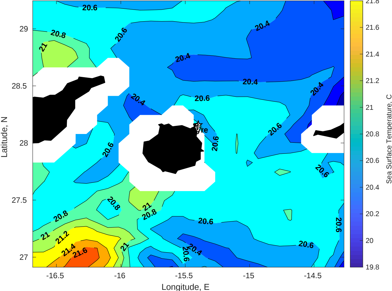
SST for Gyre at 29-May-2025 00:00:00
