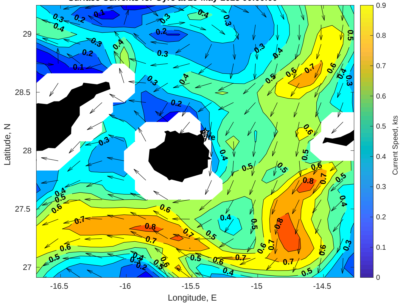
Surface Currents for Gyre at 29-May-2025 00:00:00
