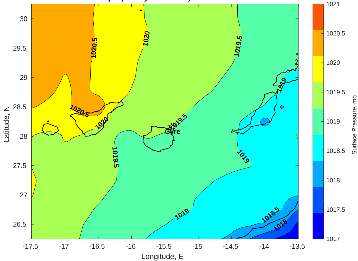
Surface Pressure (mb) for Gyre at 30-May-2025 12:00:00
