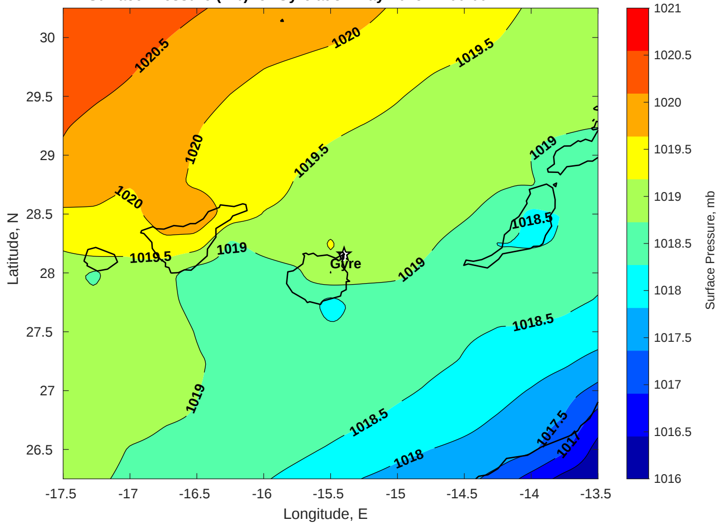
Surface Pressure (mb) for Gyre at 31-May-2025 12:00:00
