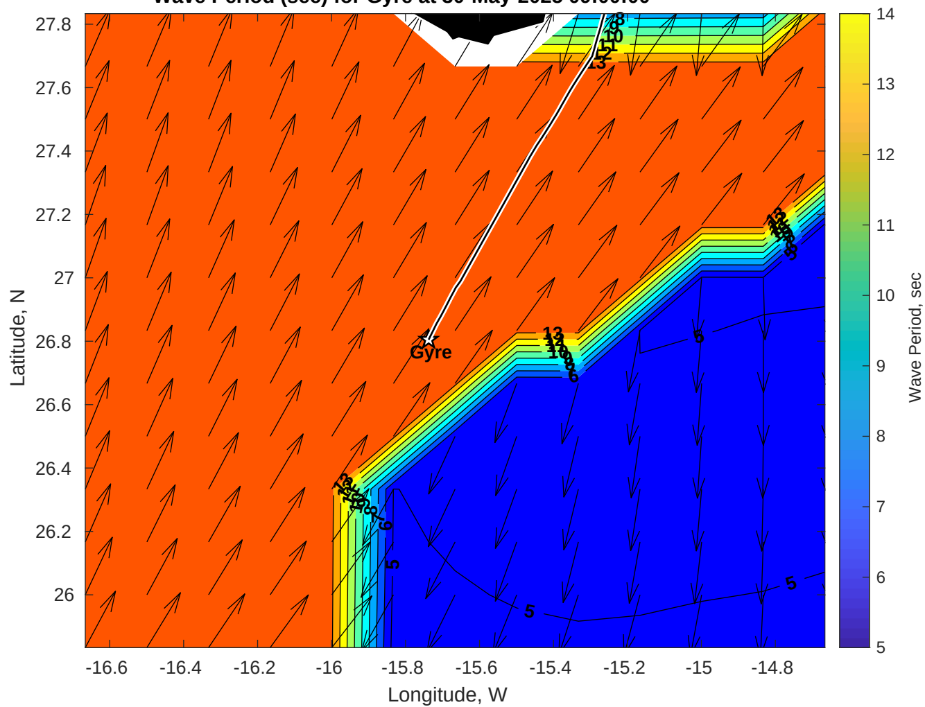
Wave Period (sec) for Gyre at 30-May-2025 09:00:00
