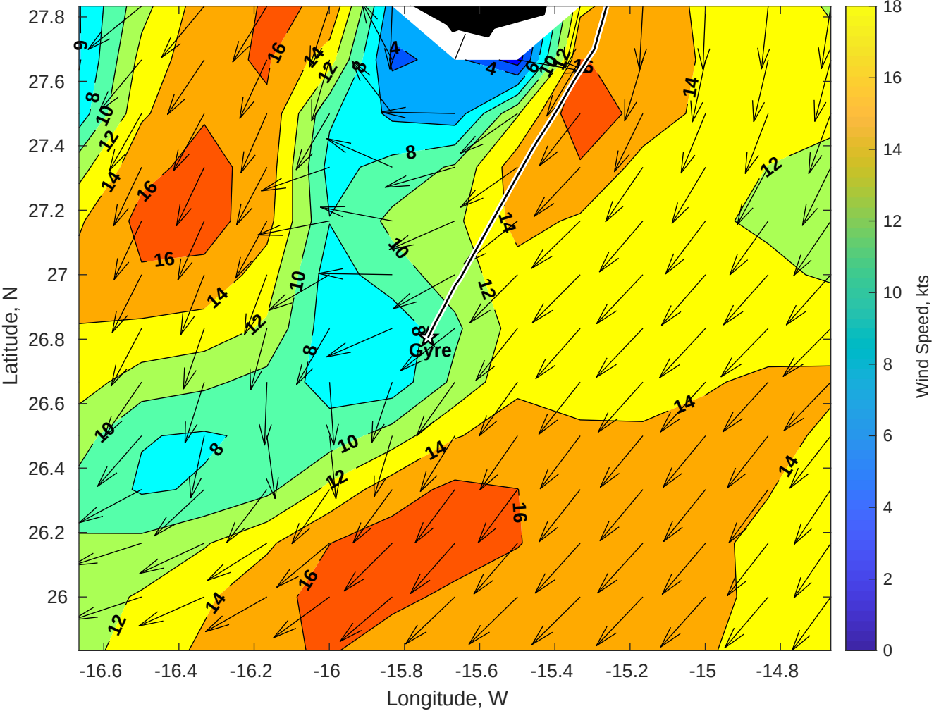
Winds (kts) for Gyre at 30-May-2025 09:00:00
