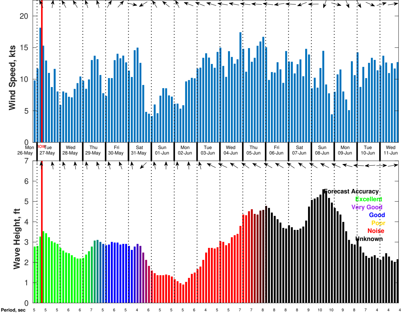
Wind & Wave Forecast for Shell Noches GC19 PPL Geotechnical from 26-May-2025 20:00:00 to 11-Jun-2025 20:00:00
