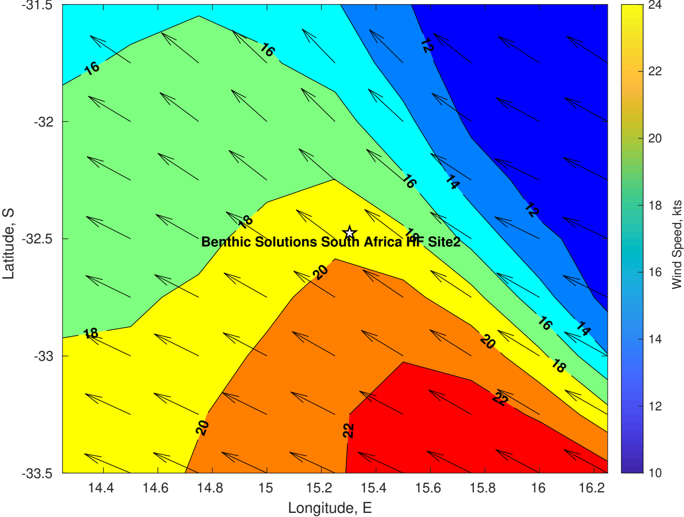
Winds (kts) for Benthic Solutions South Africa HF Site2 at 27-May-2025 09:00:00
