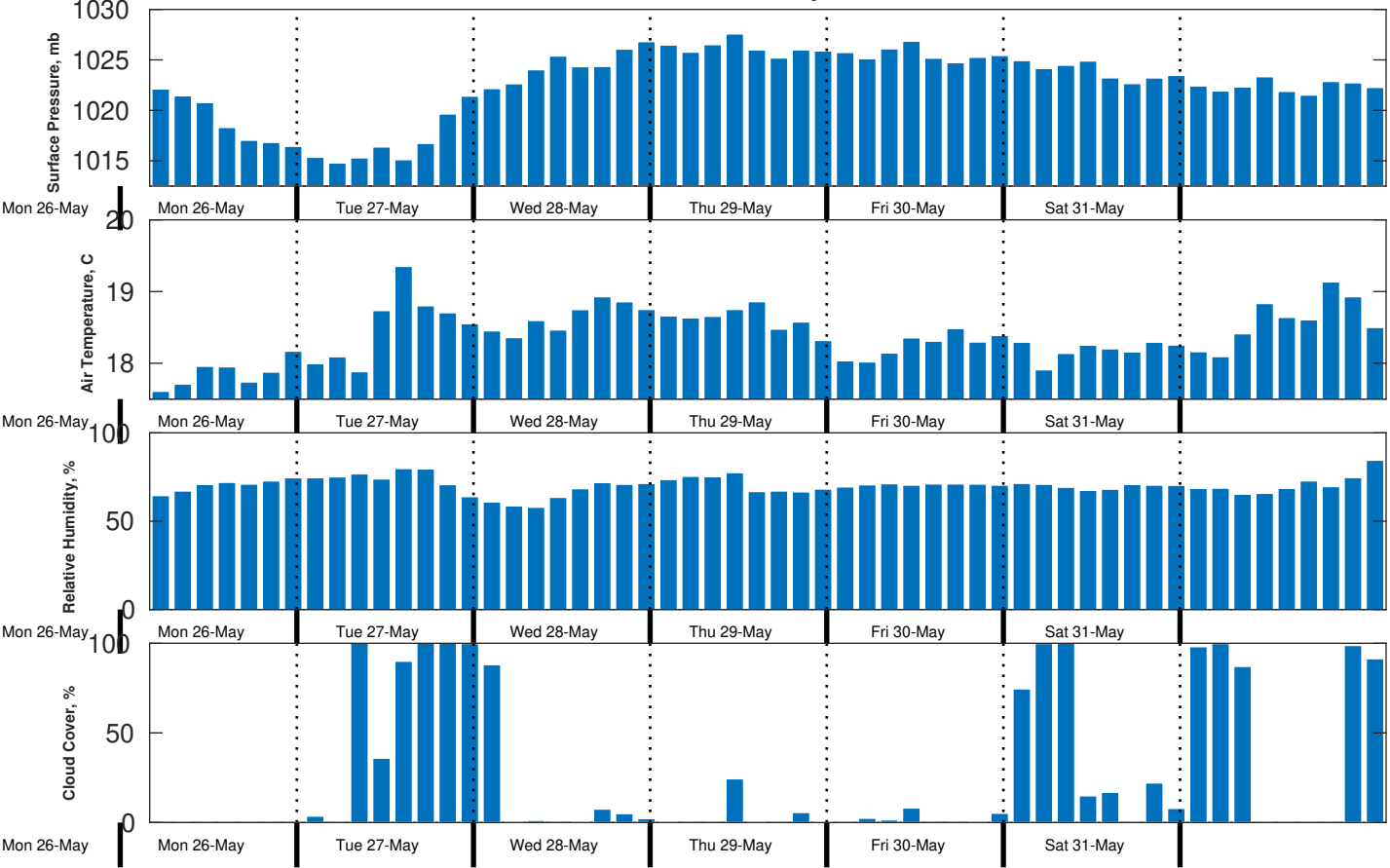
Met Forecast for Benthic Solutions South Africa HF Site2 from 27-May-2025 00:00:00 to 03-Jun-2025 00:00:00
