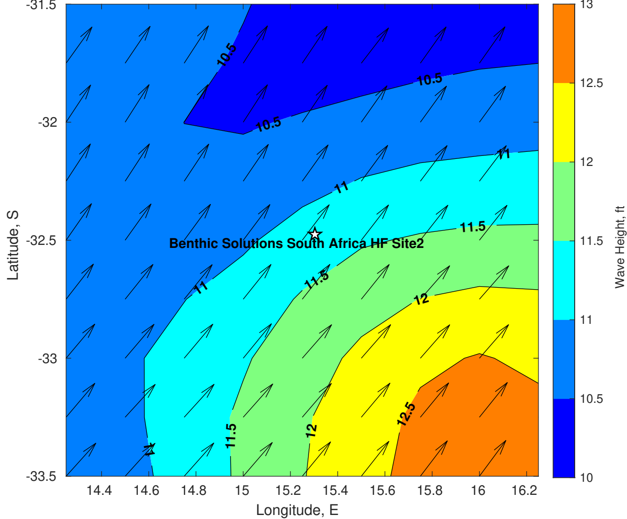
Wave Height (ft) for Benthic Solutions South Africa HF Site2 at 27-May-2025 09:00:00
