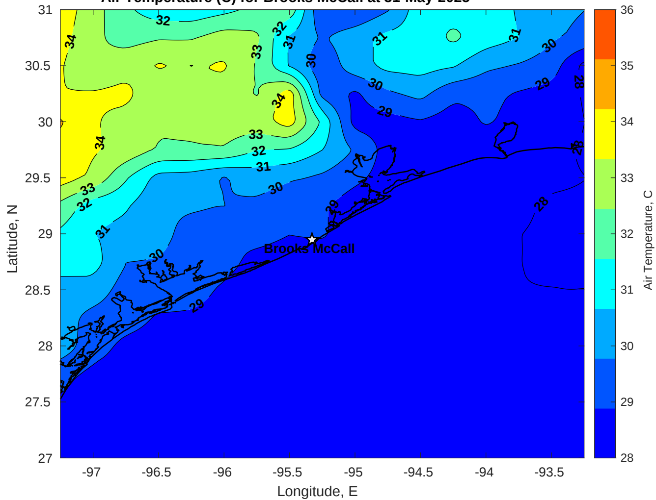
Air Temperature (C) for Brooks McCall at 31-May-2025
