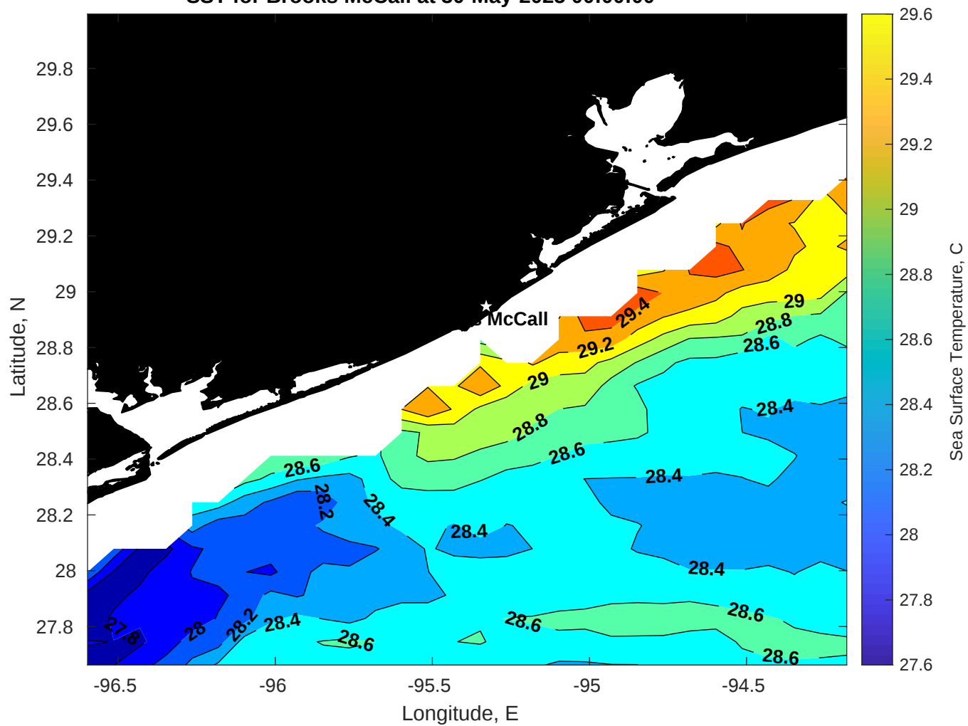
SST for Brooks McCall at 30-May-2025 00:00:00
