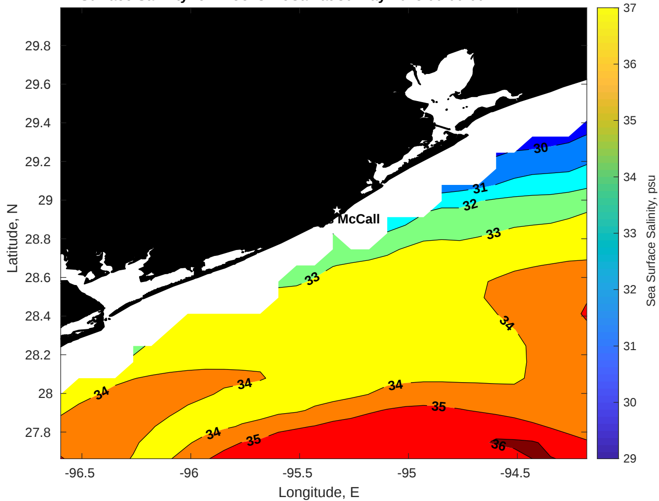
Surface Salinity for Brooks McCall at 30-May-2025 00:00:00
