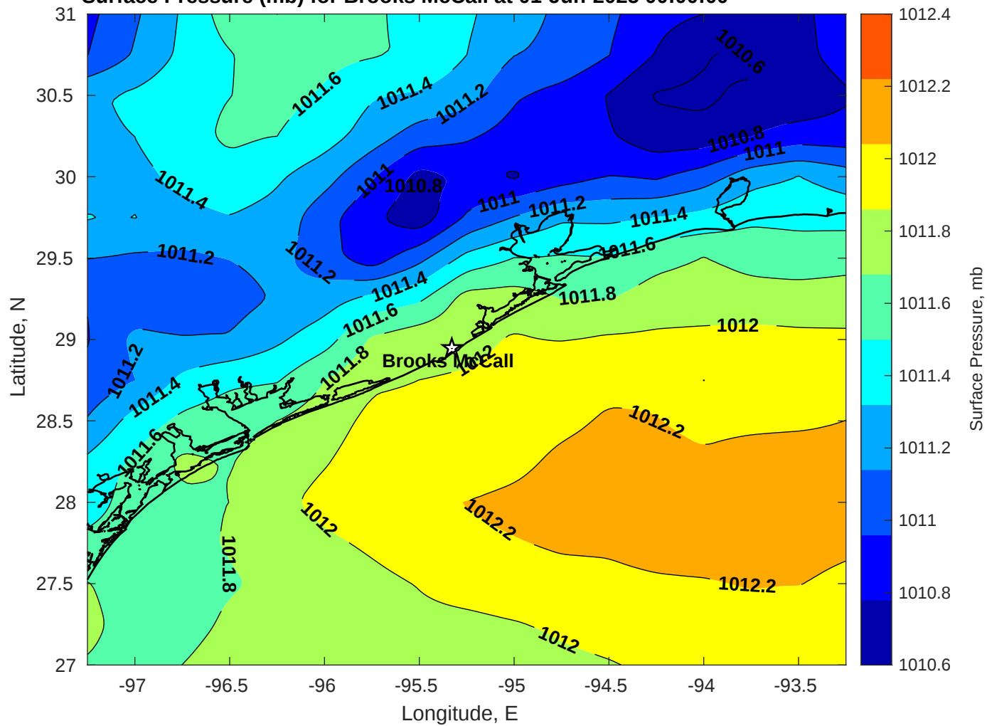
Surface Pressure (mb) for Brooks McCall at 01-Jun-2025 00:00:00
