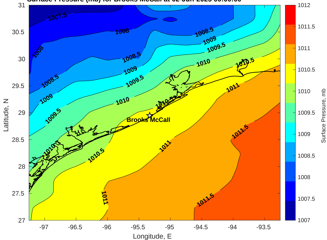
Surface Pressure (mb) for Brooks McCall at 02-Jun-2025 00:00:00
