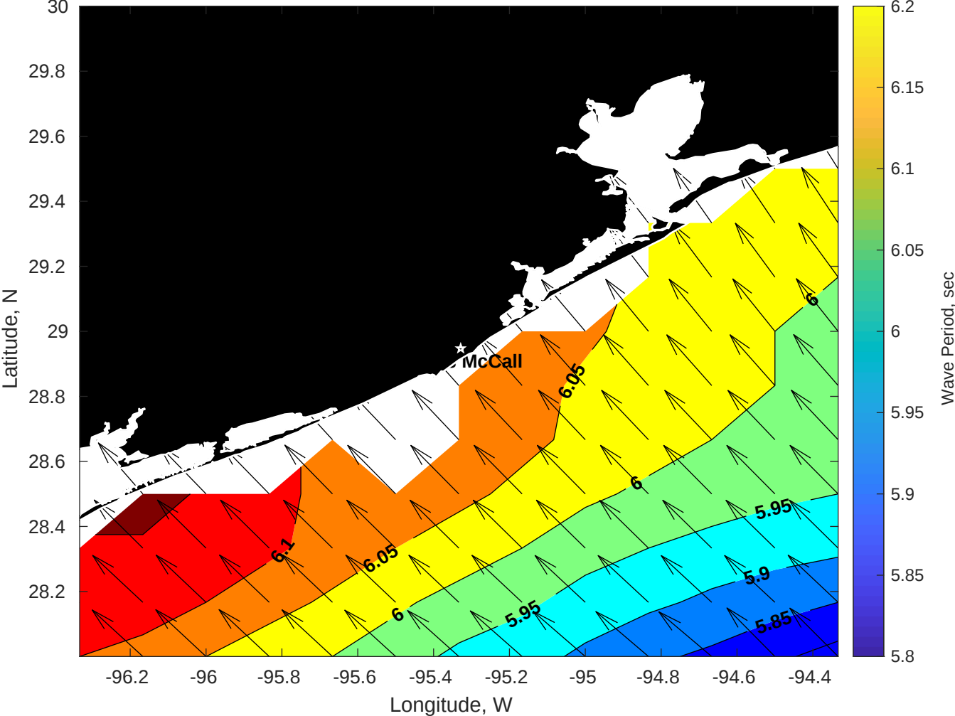
Wave Period (sec) for Brooks McCall at 31-May-2025 09:00:00
