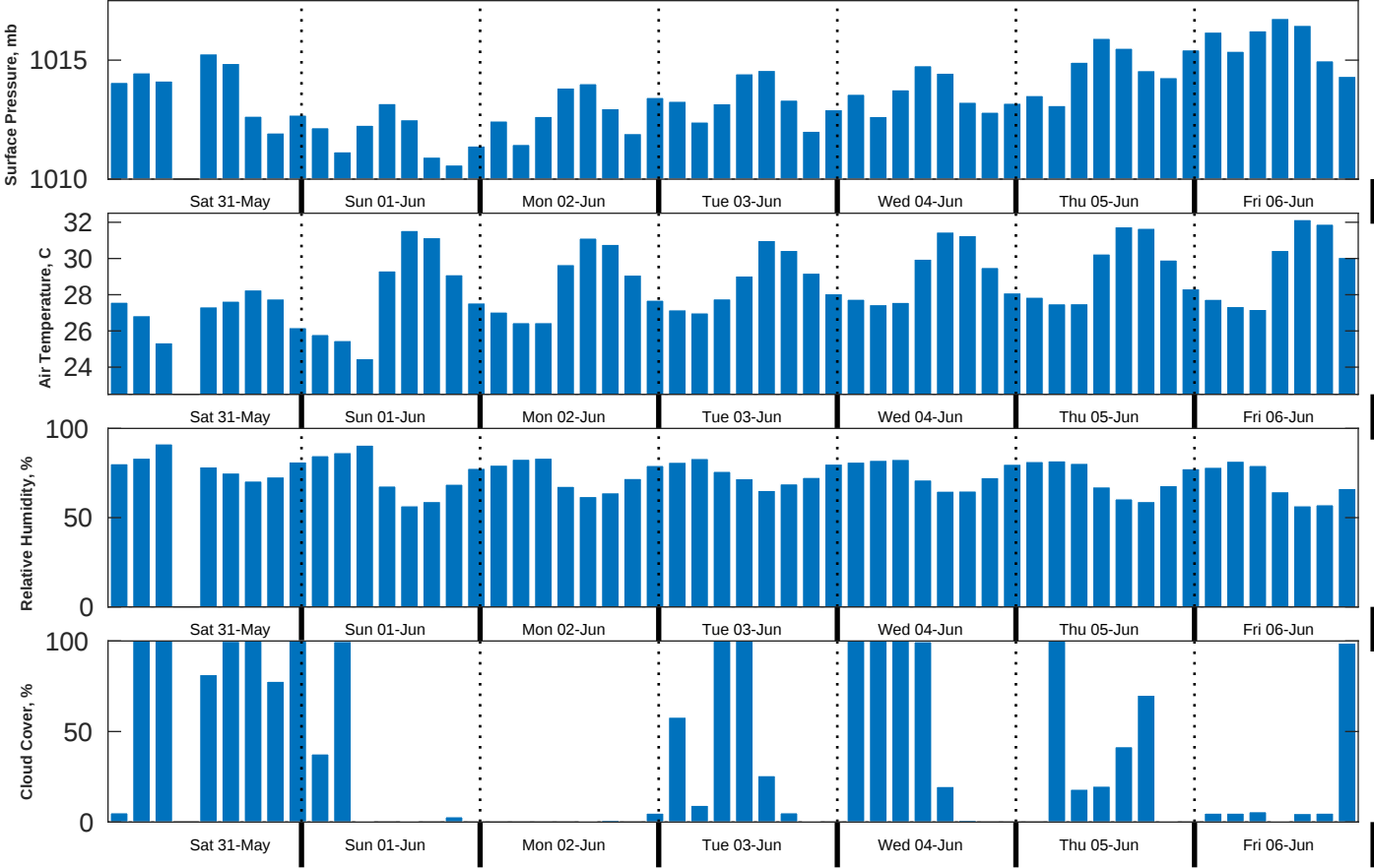
Met Forecast for Brooks McCall from 31-May-2025 00:00:00 to 07-Jun-2025 00:00:00
