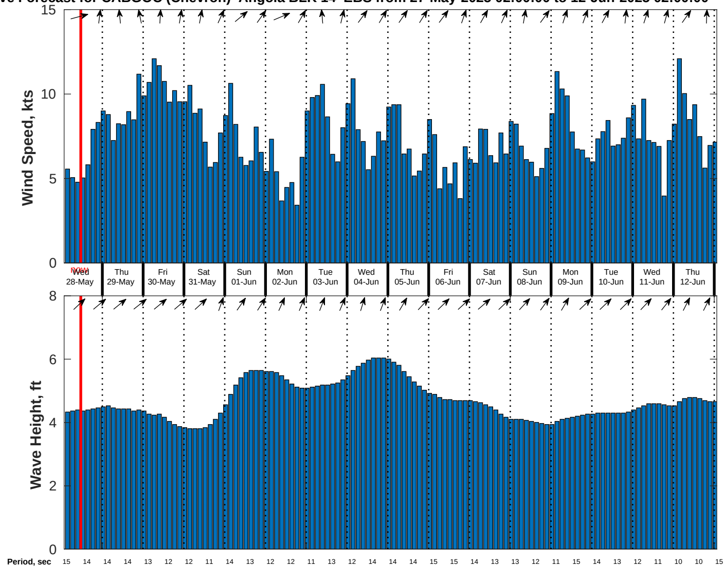
Wind & Wave Forecast for CABGOC (Chevron) Angola BLK 14 EBS from 27-May-2025 02:00:00 to 12-Jun-2025 02:00:00
