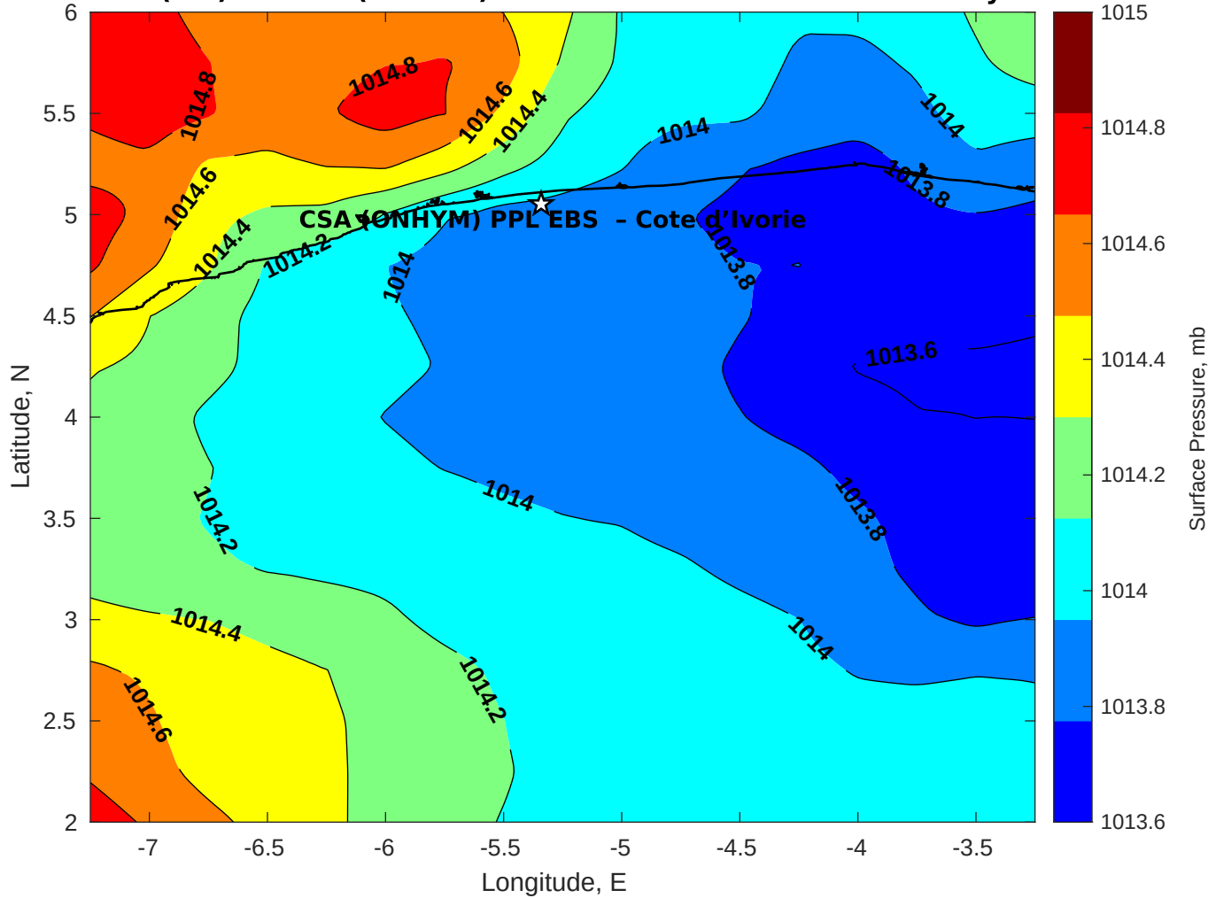
Surface Pressure (mb) for CSA (ONHYM) PPL EBS - Cote d'Ivoire at 29-May-2025 00:00:00
