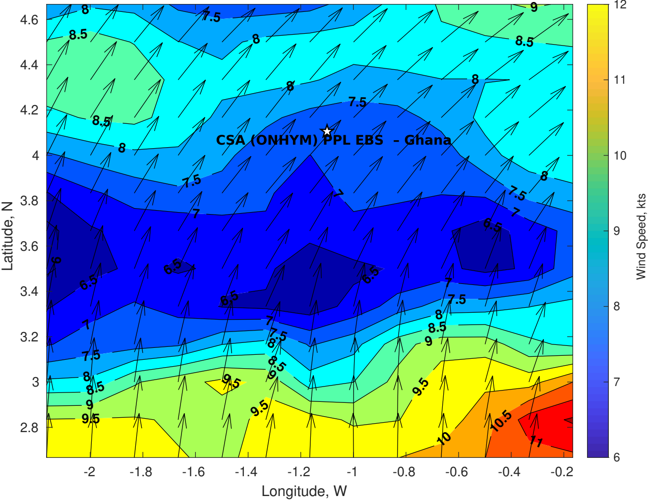
Winds (kts) for CSA (ONHYM) PPL EBS - Ghana at 27-May-2025 09:00:00
