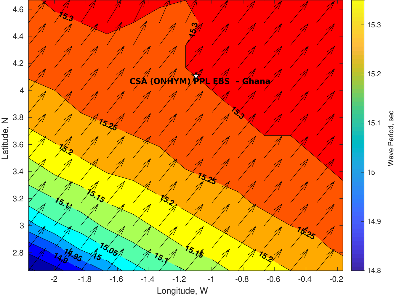
Wave Period (sec) for CSA (ONHYM) PPL EBS - Ghana at 27-May-2025 09:00:00
