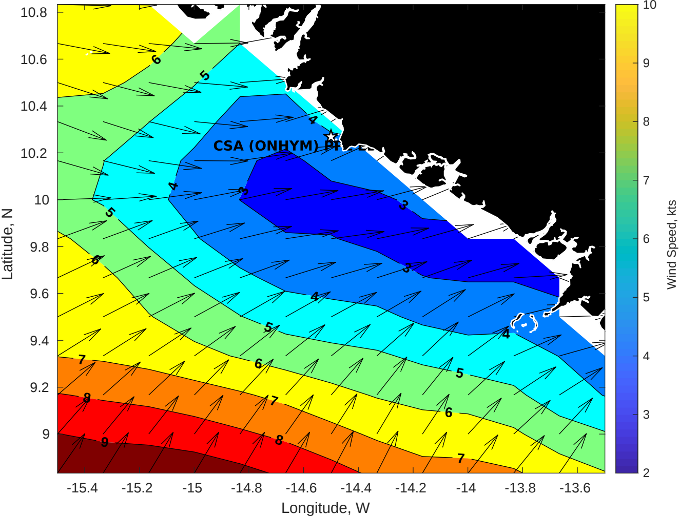
Winds (kts) for CSA (ONHYM) PPL EBS - Guinea at 27-May-2025 09:00:00
