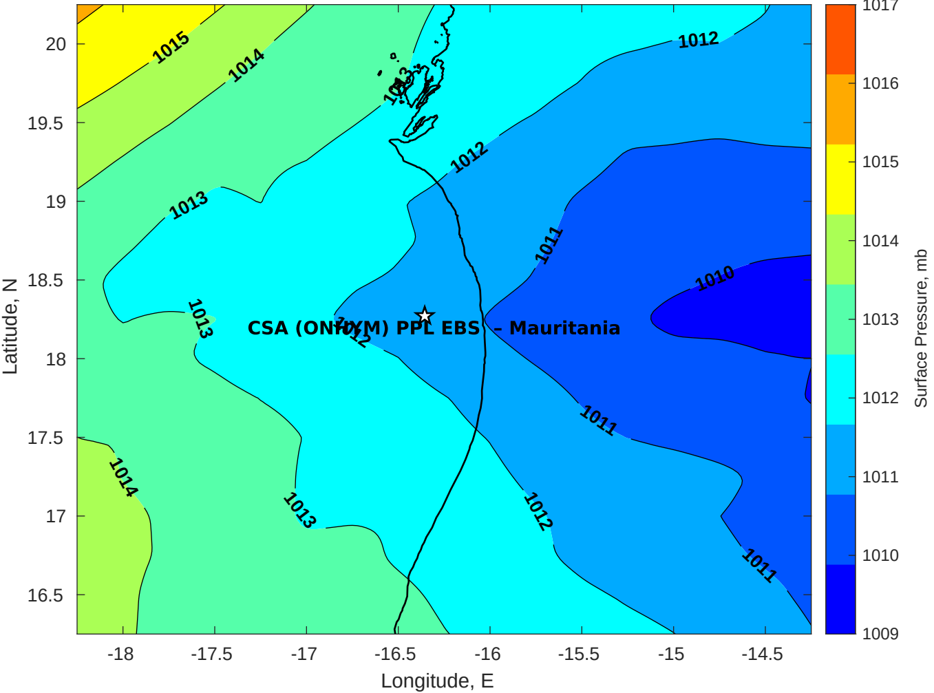
Surface Pressure (mb) for CSA (ONHYM) PPL EBS - Mauritania at 29-May-2025 00:00:00
