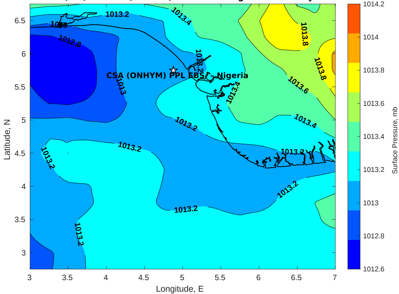
Surface Pressure (mb) for CSA (ONHYM) PPL EBS - Nigeria at 27-May-2025 00:00:00
