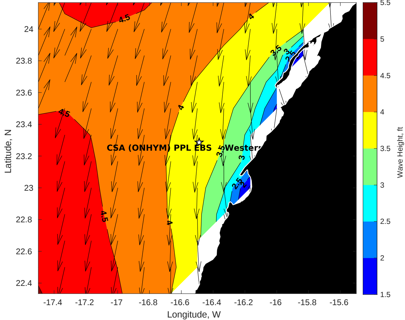
Wave Height (ft) for CSA (ONHYM) PPL EBS - Western Sahara at 27-May-2025 09:00:00
