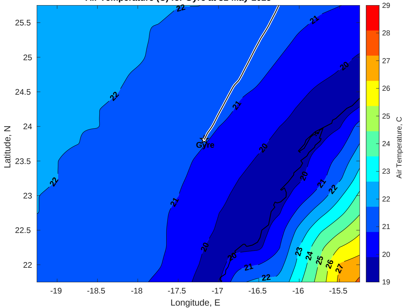
Air Temperature (C) for Gyre at 31-May-2025
