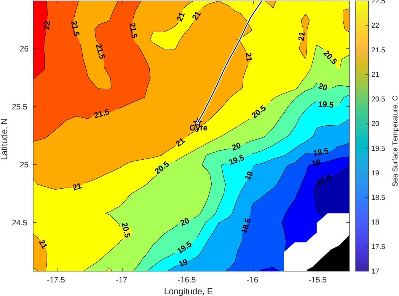
SST for Gyre at 30-May-2025 00:00:00
