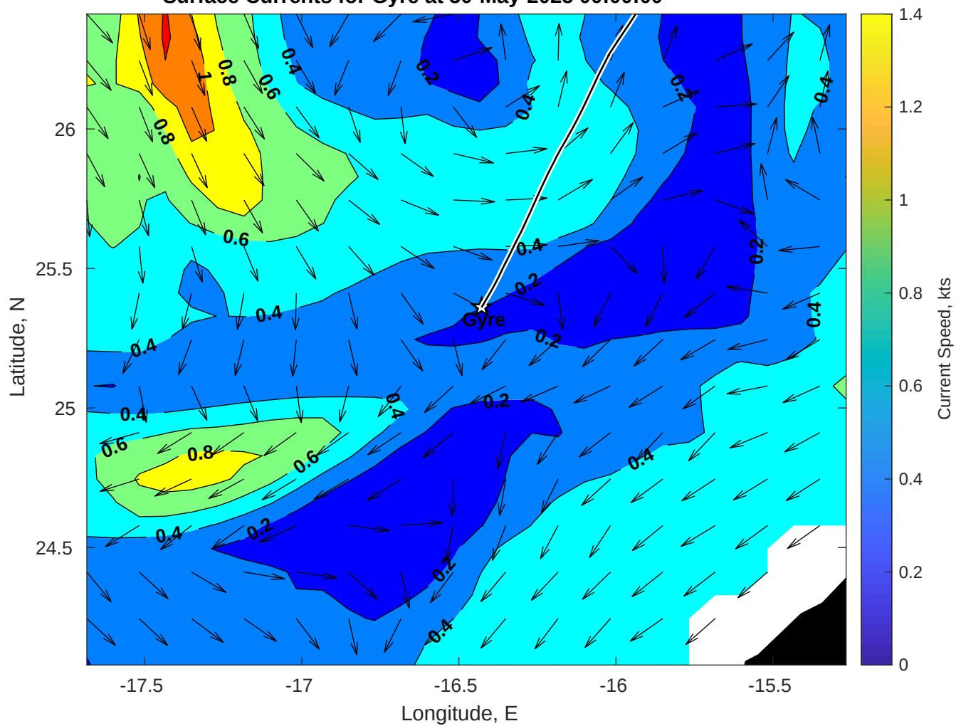
Surface Currents for Gyre at 30-May-2025 00:00:00
