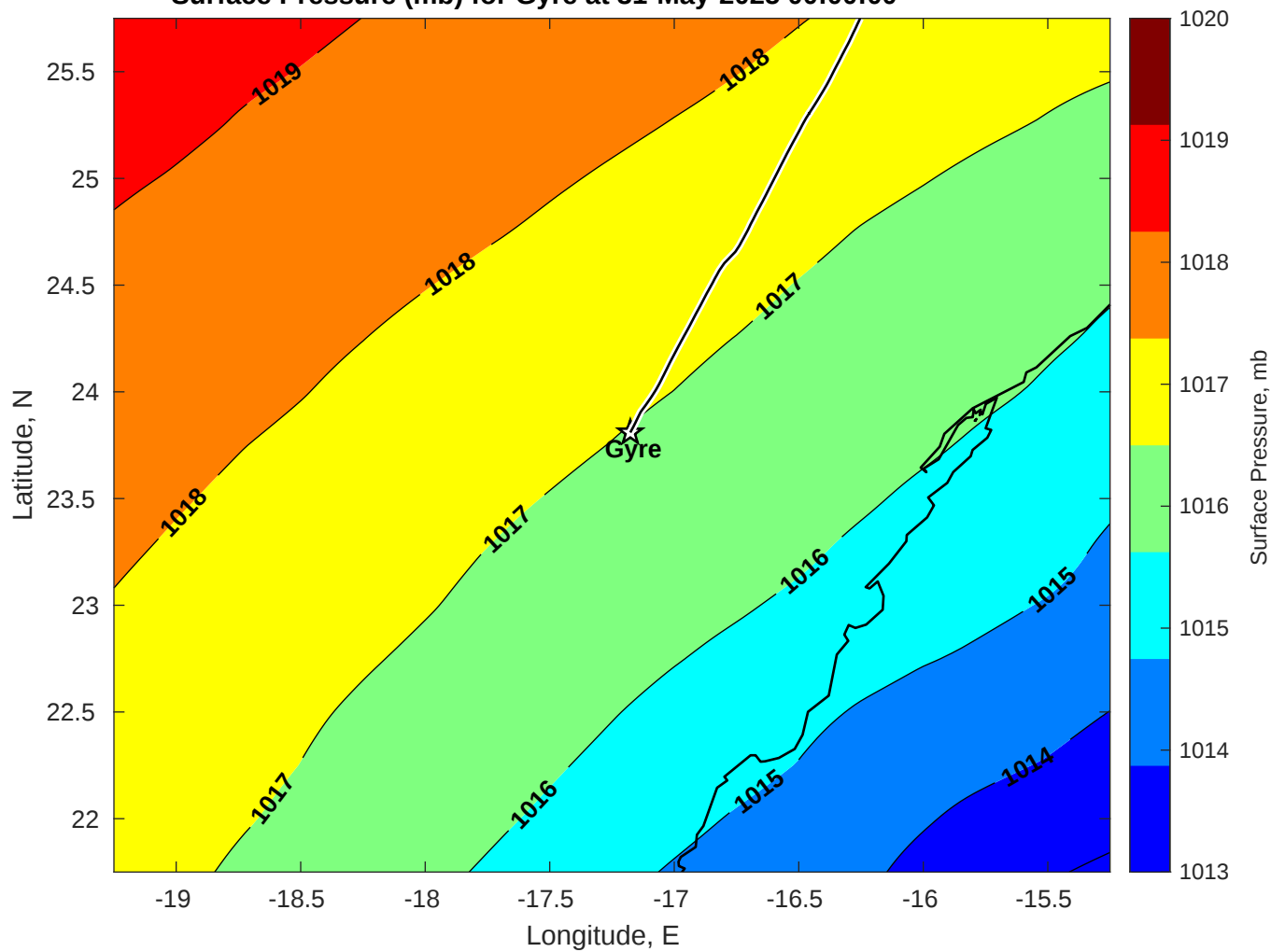
Surface Pressure (mb) for Gyre at 31-May-2025 00:00:00
