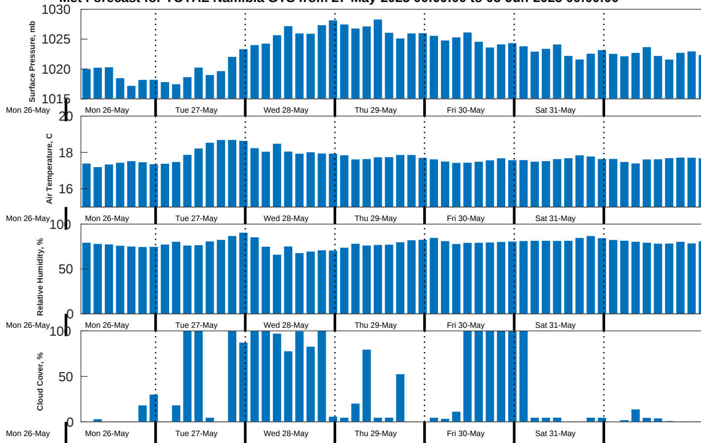
Met Forecast for TOTAL Namibia GTS from 27-May-2025 00:00:00 to 03-Jun-2025 00:00:00
