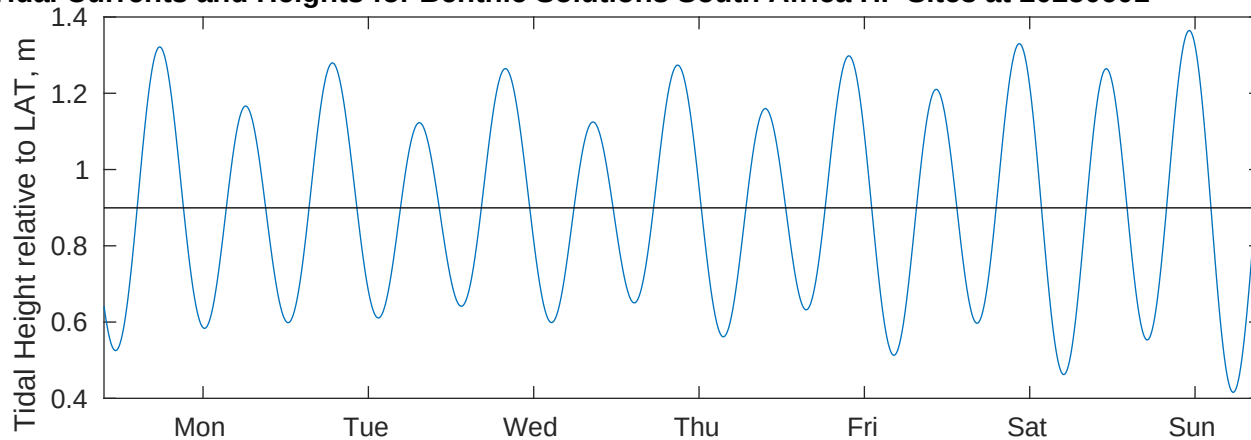
Tidal Currents and Heights for Benthic Solutions South Africa HF Site3 at 20250601
