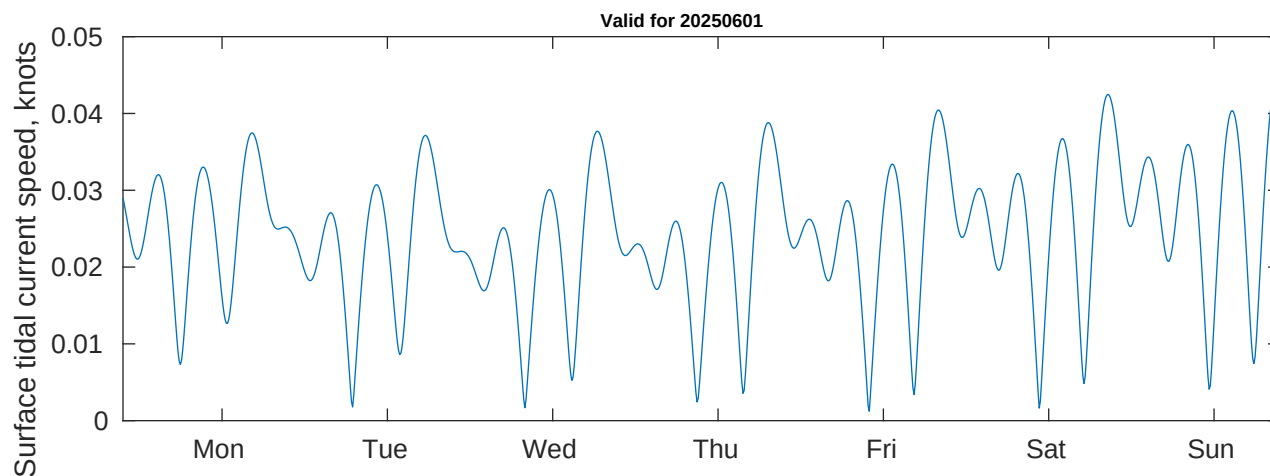
Tidal Currents and Heights for Benthic Solutions South Africa HF Site3 at 20250601
