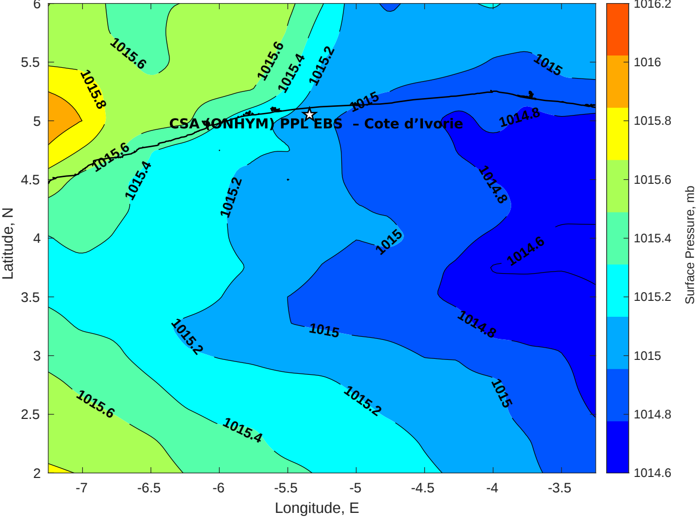
Surface Pressure (mb) for CSA (ONHYM) PPL EBS - Cote d'Ivoire at 03-Jun-2025 00:00:00
