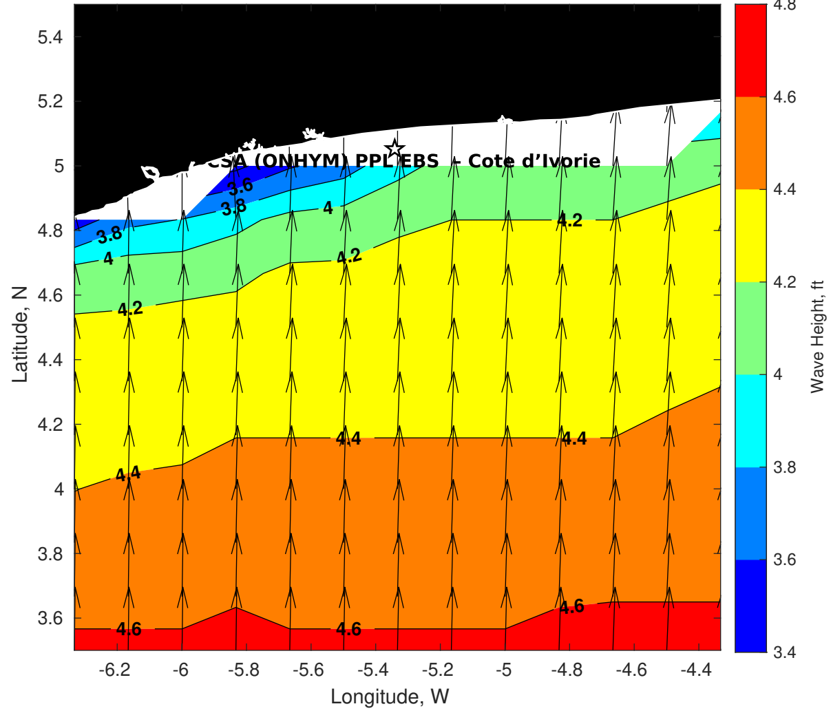
Wave Height (ft) for CSA (ONHYM) PPL EBS - Cote d'Ivoire at 01-Jun-2025 09:00:00
