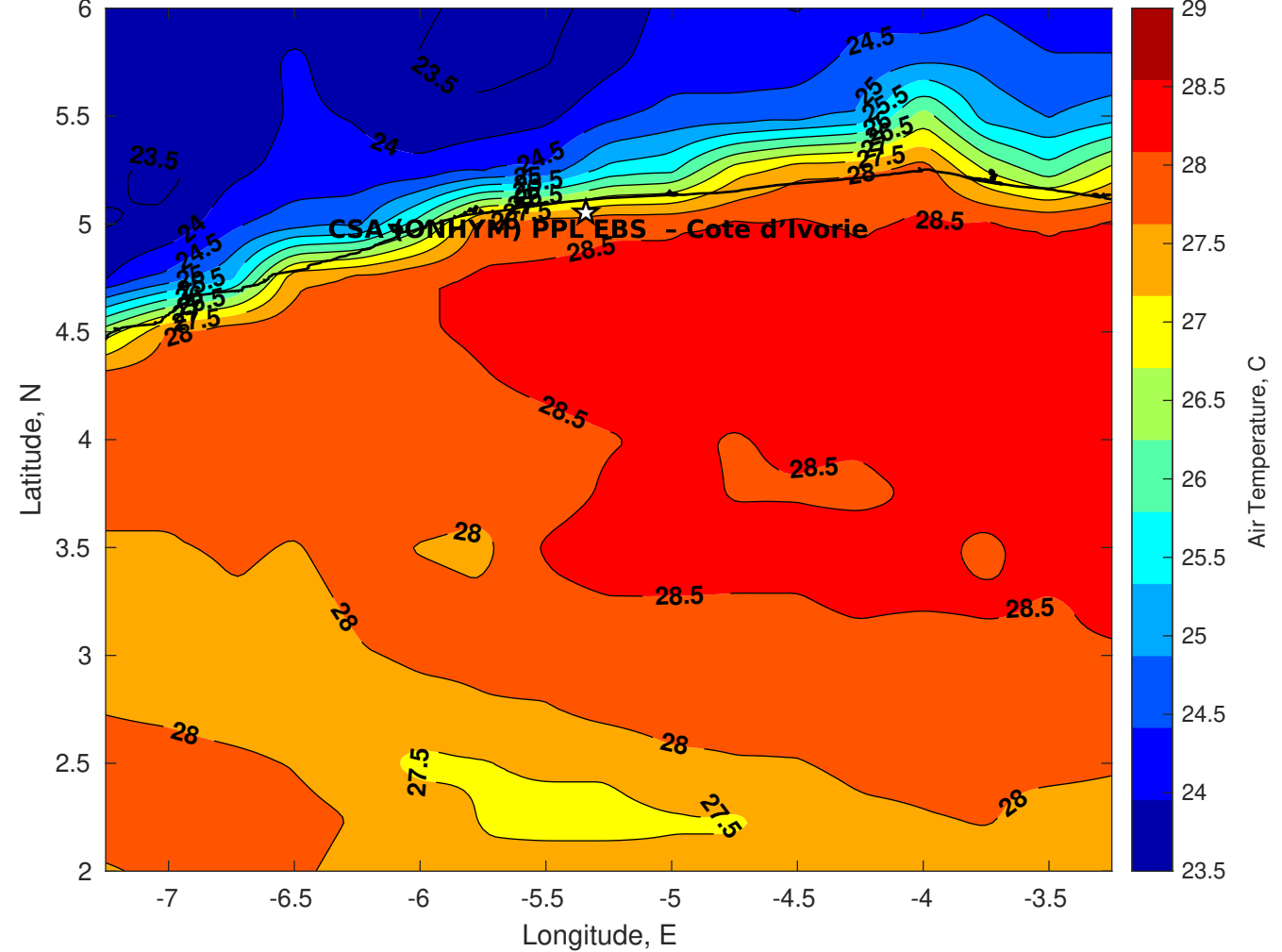
Air Temperature (C) for CSA (ONHYM) PPL EBS - Cote d'Ivoire at 01-Jun-2025
