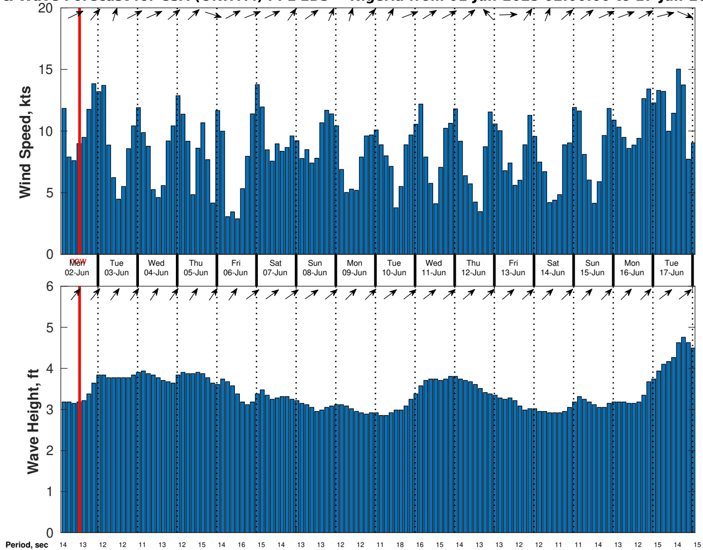
Wind & Wave Forecast for CSA (ONHYM) PPL EBS - Nigeria from 01-Jun-2025 02:00:00 to 17-Jun-2025 02:00:00
