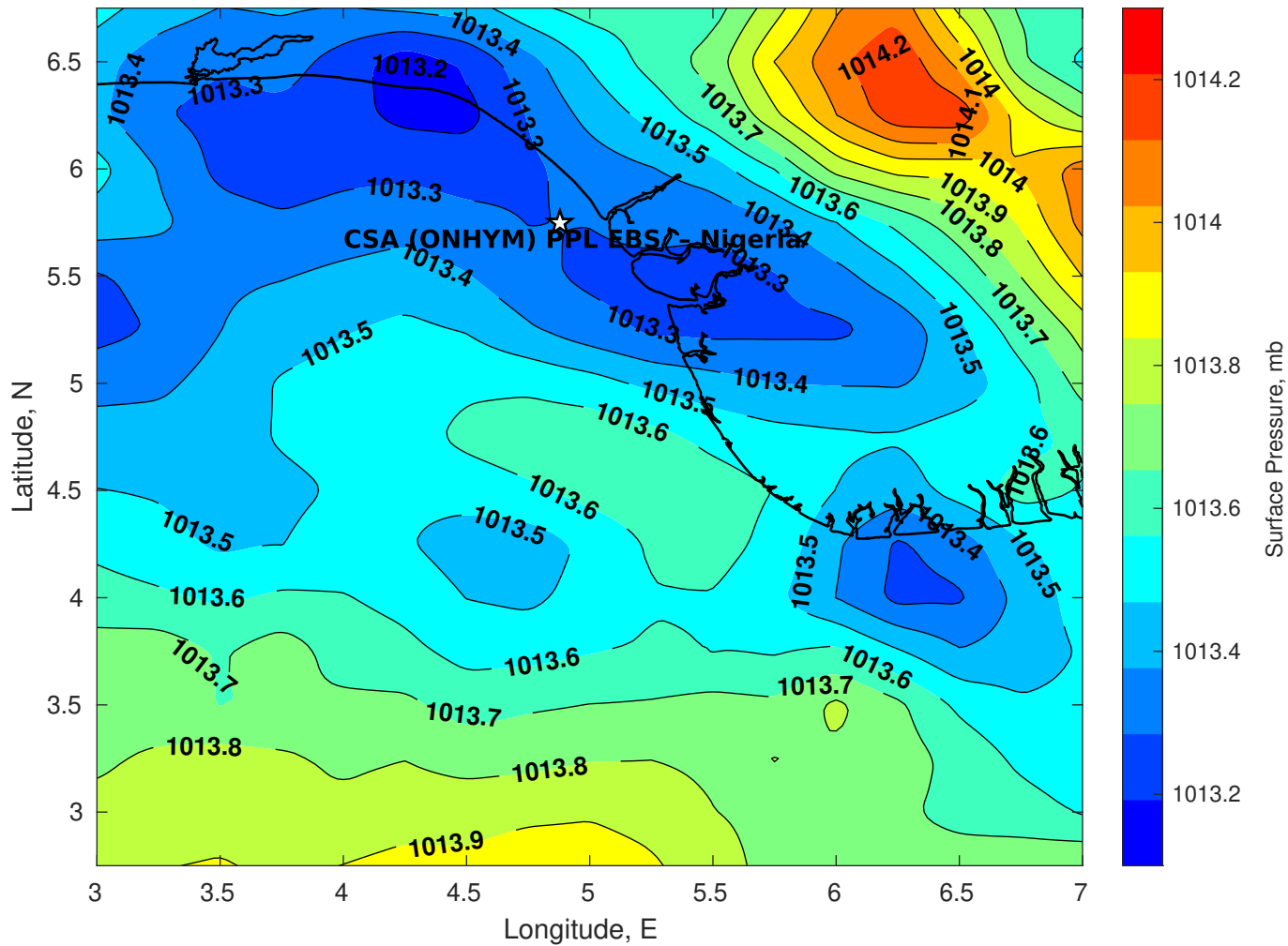
Surface Pressure (mb) for CSA (ONHYM) PPL EBS - Nigeria at 01-Jun-2025 00:00:00
