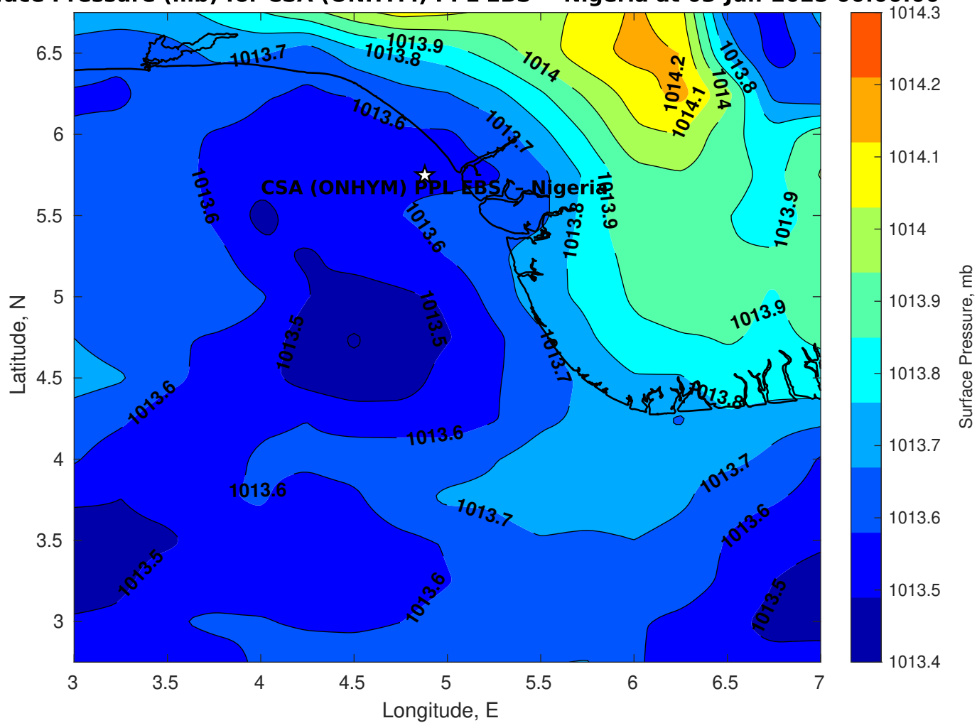
Surface Pressure (mb) for CSA (ONHYM) PPL EBS - Nigeria at 03-Jun-2025 00:00:00
