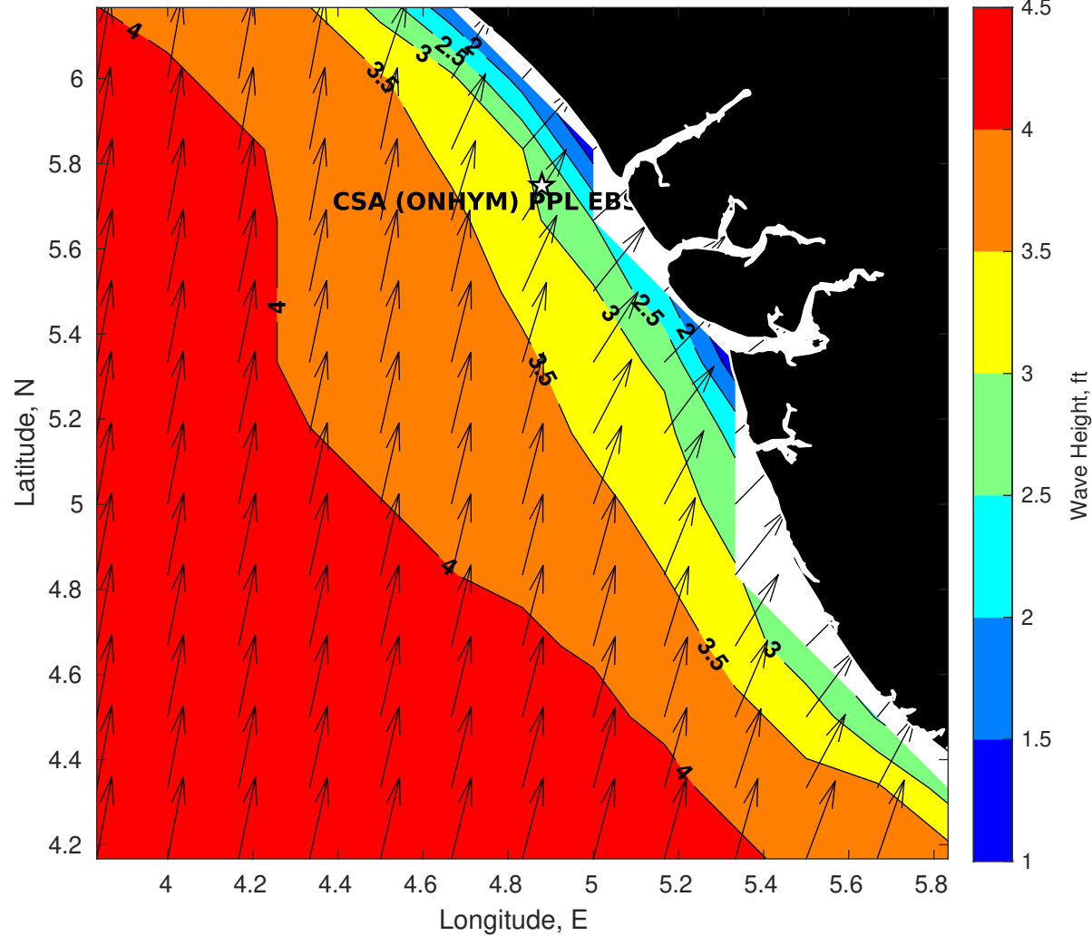
Wave Height (ft) for CSA (ONHYM) PPL EBS - Nigeria at 01-Jun-2025 09:00:00
