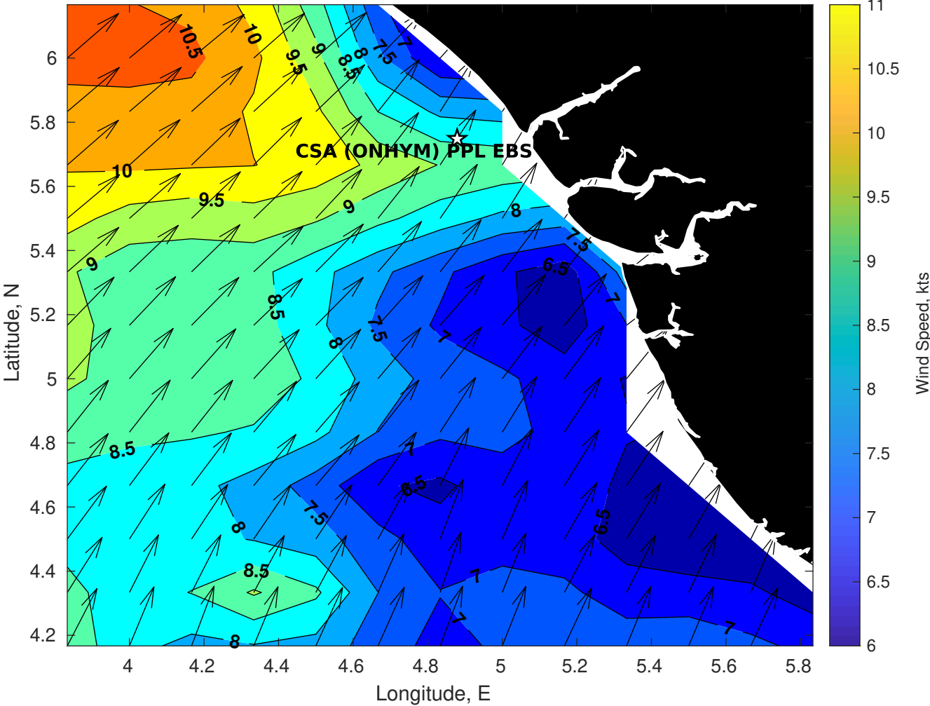
Winds (kts) for CSA (ONHYM) PPL EBS - Nigeria at 01-Jun-2025 09:00:00
