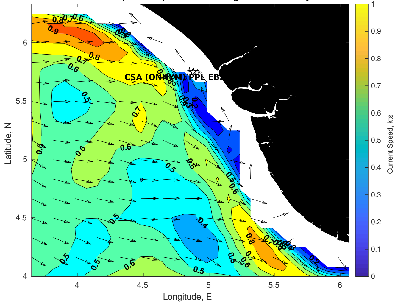
Surface Currents for CSA (ONHYM) PPL EBS - Nigeria at 26-May-2025 00:00:00
