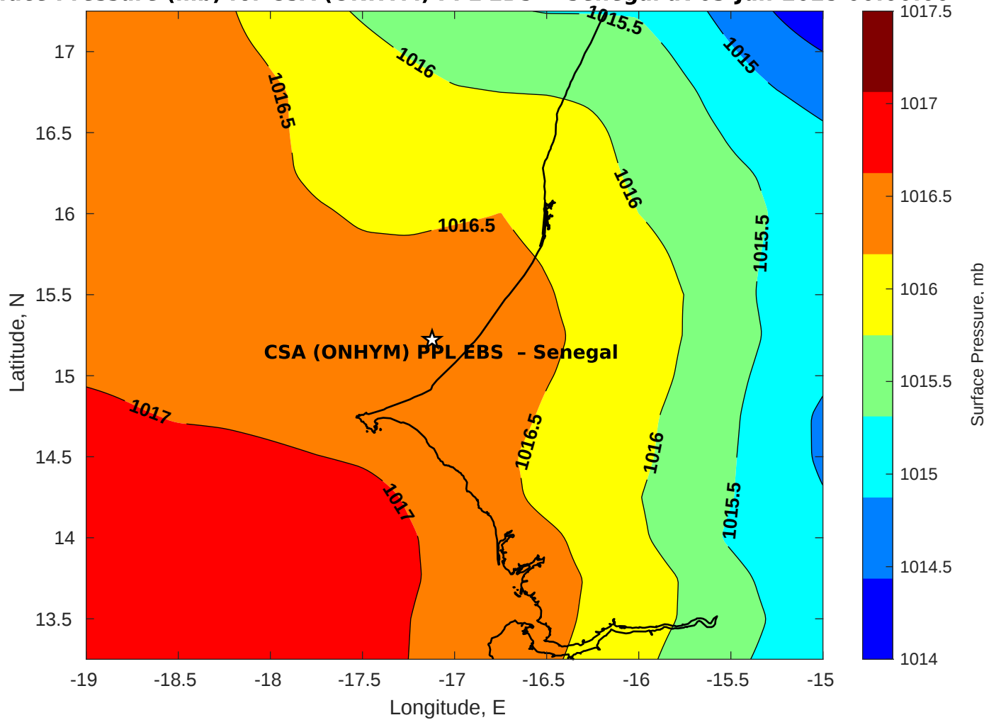
Surface Pressure (mb) for CSA (ONHYM) PPL EBS - Senegal at 03-Jun-2025 00:00:00
