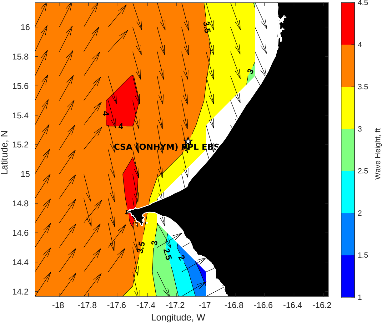
Wave Height (ft) for CSA (ONHYM) PPL EBS - Senegal at 01-Jun-2025 09:00:00
