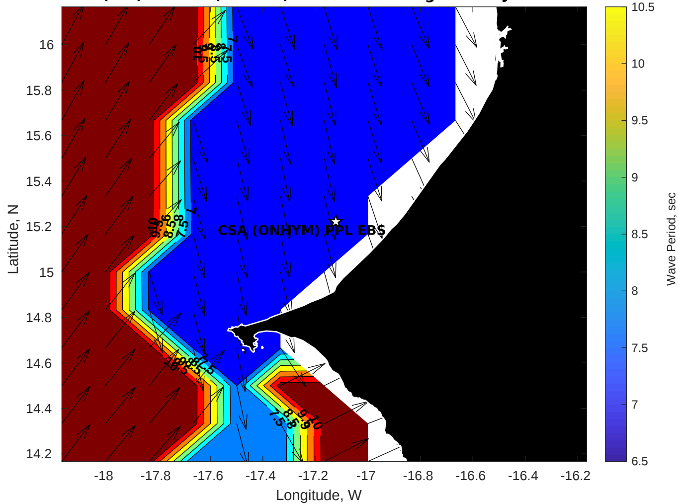
Wave Period (sec) for CSA (ONHYM) PPL EBS - Senegal at 01-Jun-2025 09:00:00
