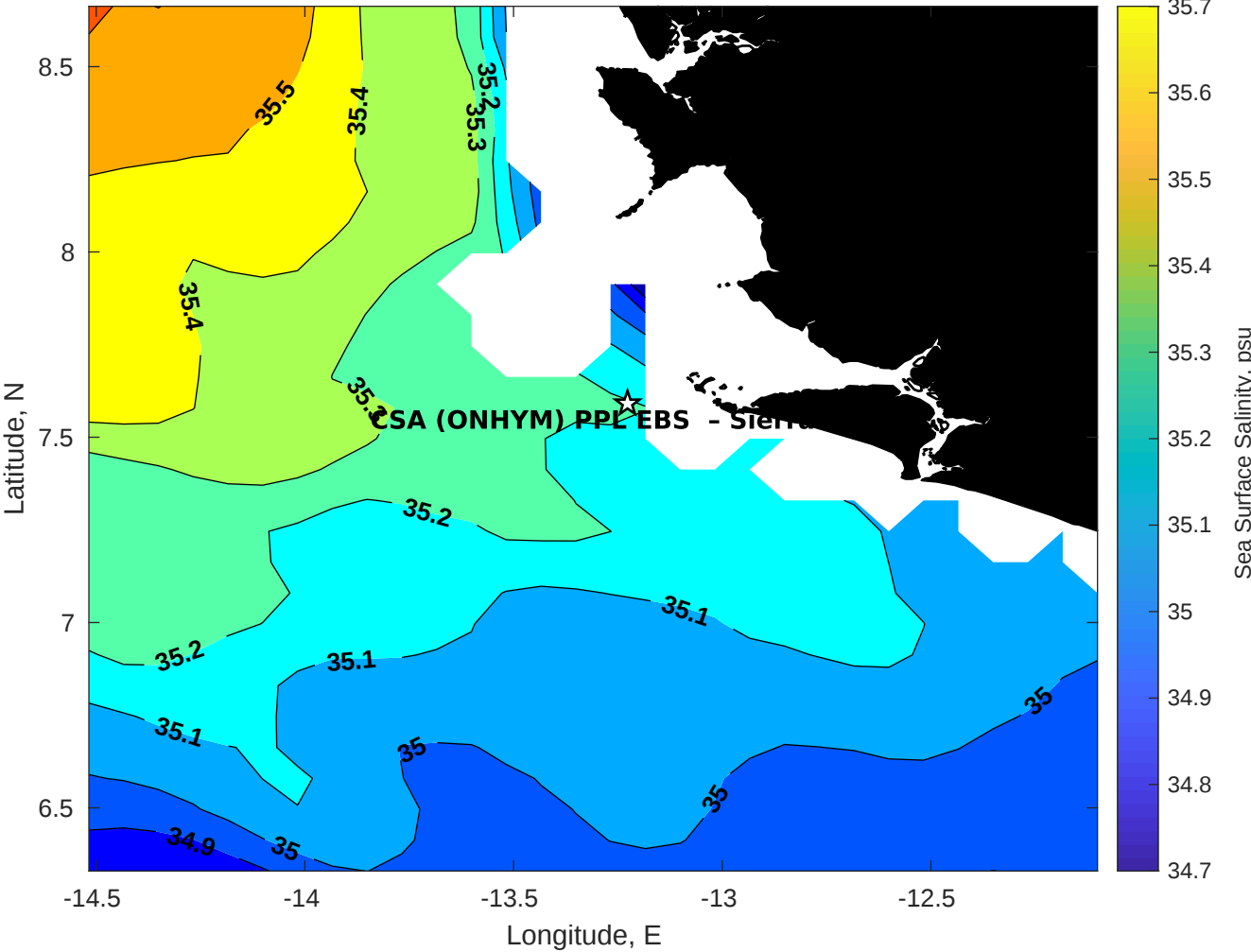
Surface Salinity for CSA (ONHYM) PPL EBS - Sierra Leone at 26-May-2025 00:00:00
