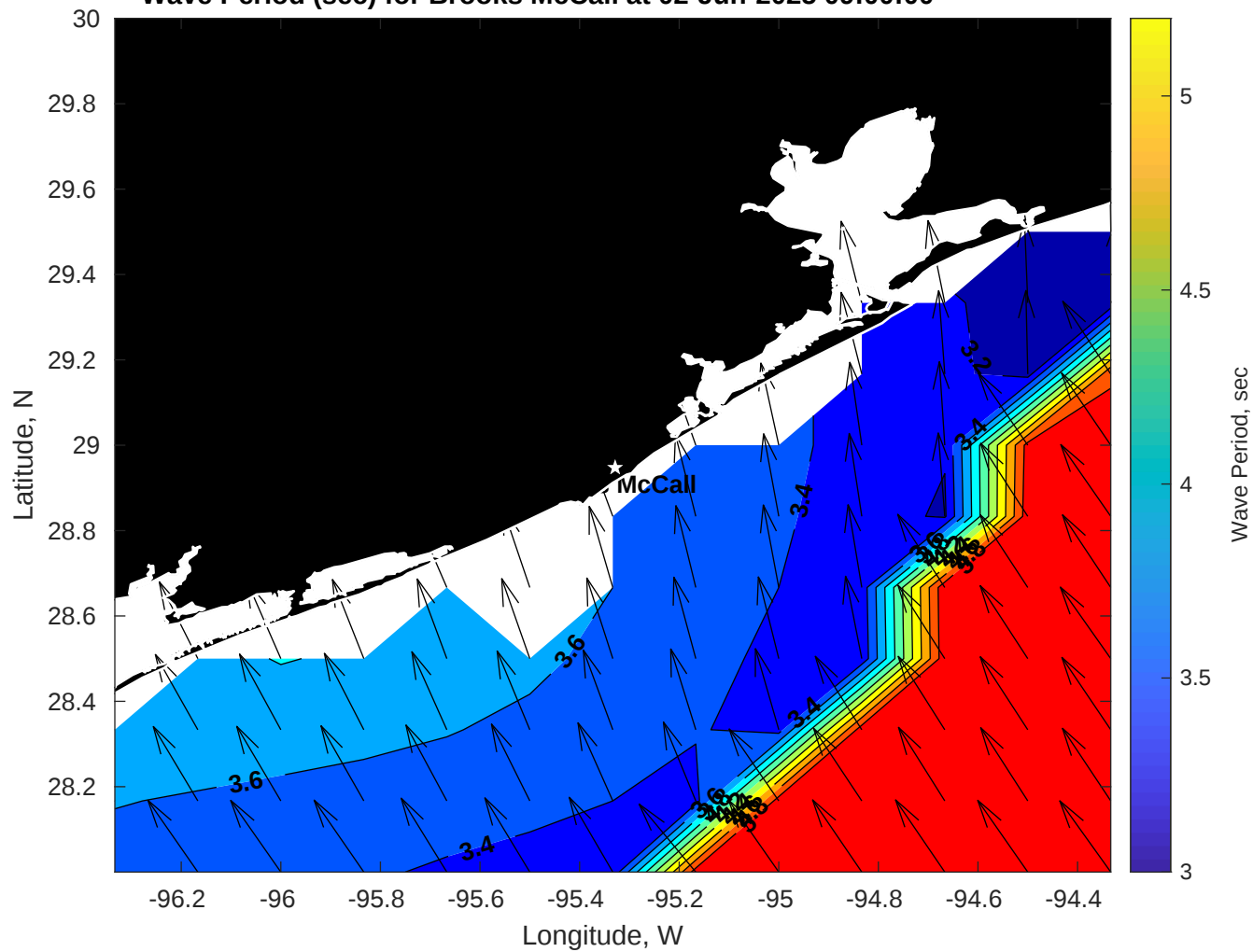
Wave Period (sec) for Brooks McCall at 02-Jun-2025 09:00:00
