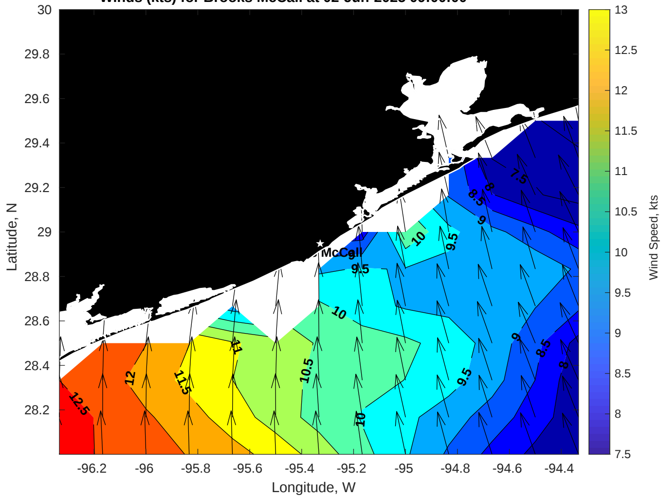
Winds (kts) for Brooks McCall at 02-Jun-2025 09:00:00
