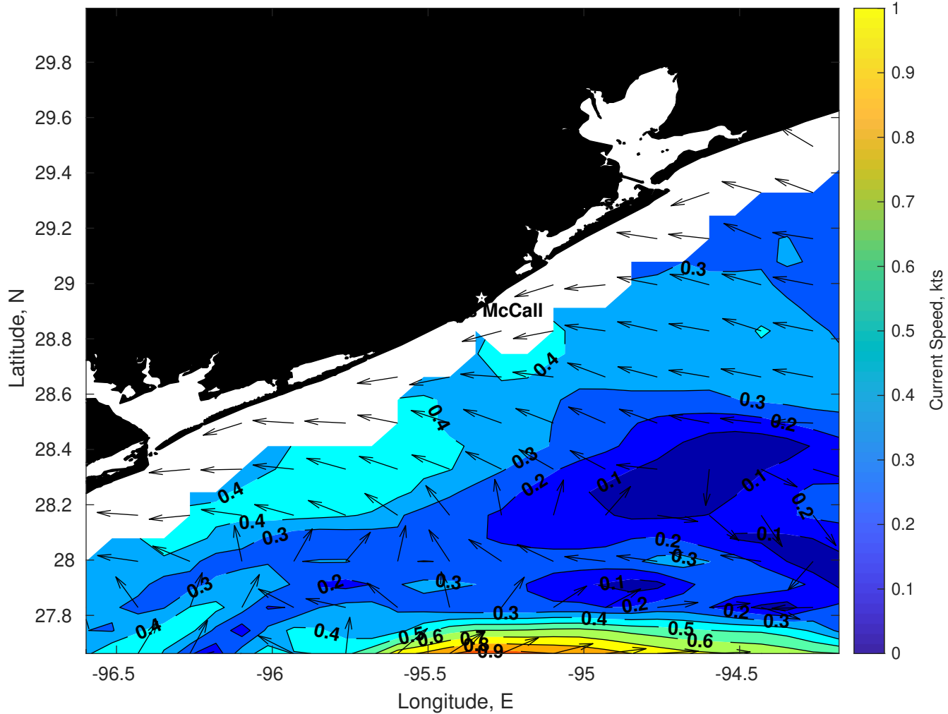
Surface Currents for Brooks McCall at 01-Jun-2025 00:00:00
